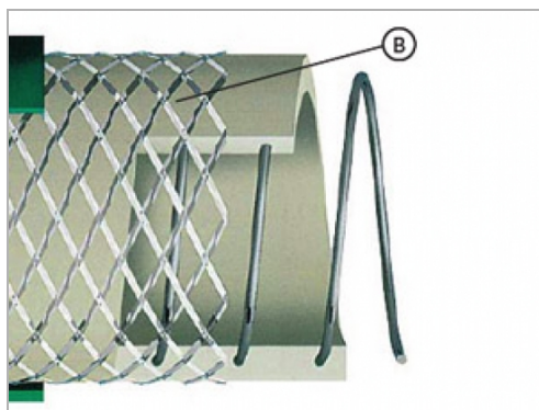
Reinforcement: Polyester high tenacity yarn
